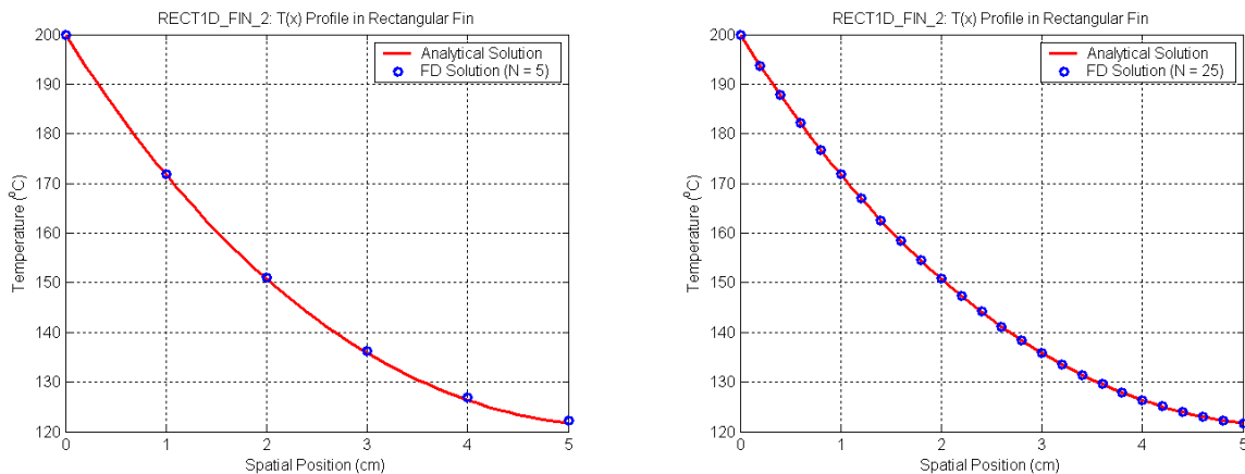
Fig. 2 Fin temperature profile -- comparison of the analytical and FD methods.
